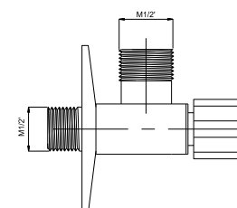
ANGLE VALVE M1/2"xM1/2" 662011
