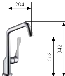
Single lever kitchen mixer with swivel spout Ref. 39850, -000, -800 for open water heaters Ref. 39852, -000, -800
