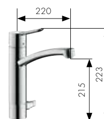
Single lever kitchen mixer with shut-off valve Ref. 31783000
