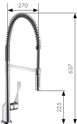
Semi-Pro Single lever kitchen mixer Ref. 39840, -000, -800
