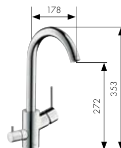
Single lever kitchen mixer with swivel spout with shut-off valve Ref. 14875000
