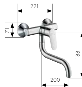
Single lever kitchen mixer for wall installation Ref. 31825000
