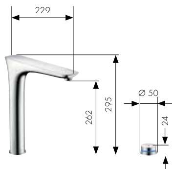
2-hole electronic kitchen mixer Ref. 15805, -000, -800
